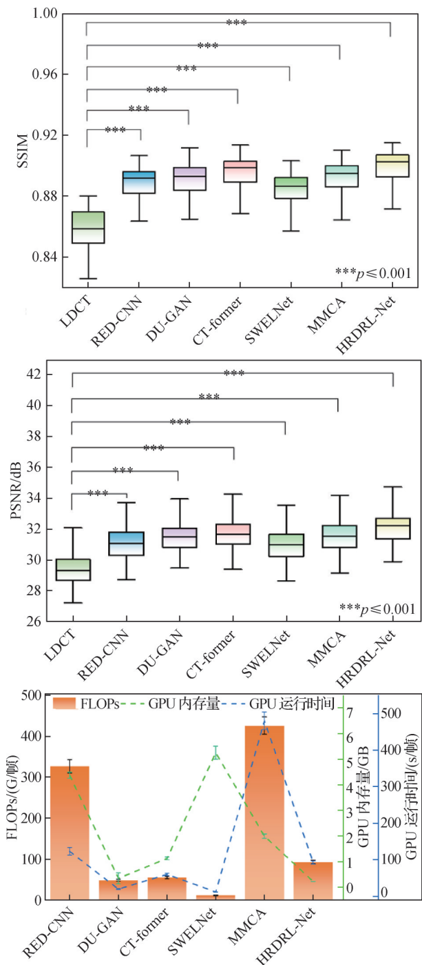
图 10 对 Piglet 测试集中全部样本进行图像重建的评价指标统计结果 Fig. 10 Statistical results of the evaluation indicators for image reconstruction of all samples in the Piglet testset
