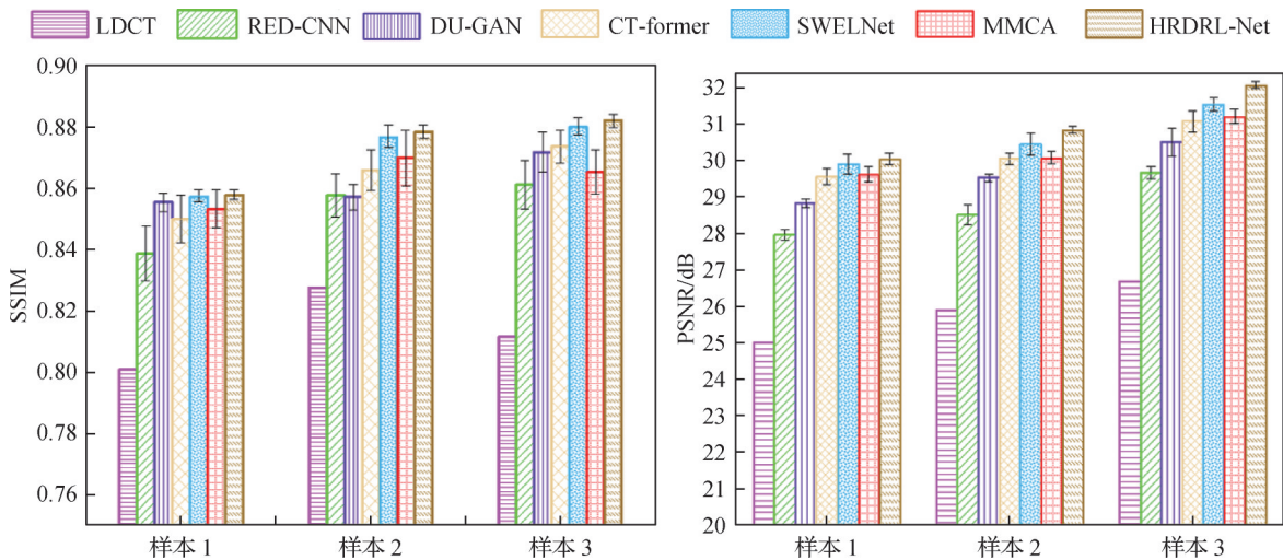
图 7 对 Mayo 测试集中随机选取的 3 个样本图像重建结果的评价指标 Fig. 7 Evaluation metrics for image reconstruction results of three randomly selected samples from the Mayo testset
